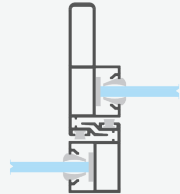
25mm FINE INTERLOCK
