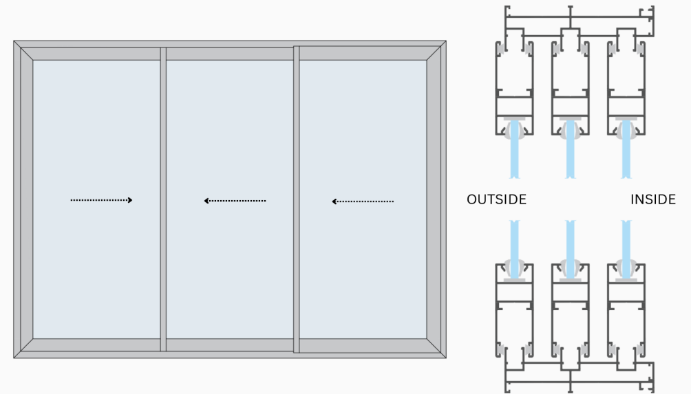
25mm FINE 3 TRACK SLIDING WINDOW
