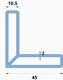
CORNER ANGLE 10.5 Section Number - SA 66 Weight ( KG/M ) - 0.956
