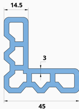
CRIMP ANGLE 14.5 Section Number - SA 95 Weight ( KG/M ) - 1.55
