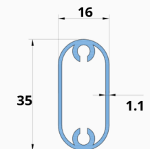
OVAL GRILL Section Number - SA 23 Weight ( KG/M ) - 0.328
