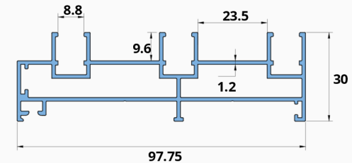
3 TRACK Section Number - SA 102 Weight ( KG/M ) - 1.078
