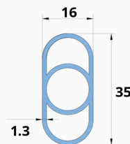
OVAL 35 GRILL Section Number - SA 04 Weight ( KG/M ) - 0.354
