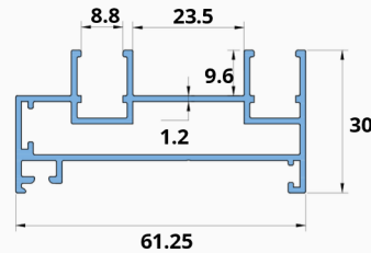
2 TRACK Section Number - SA 101 Weight ( KG/M ) - 0.707
