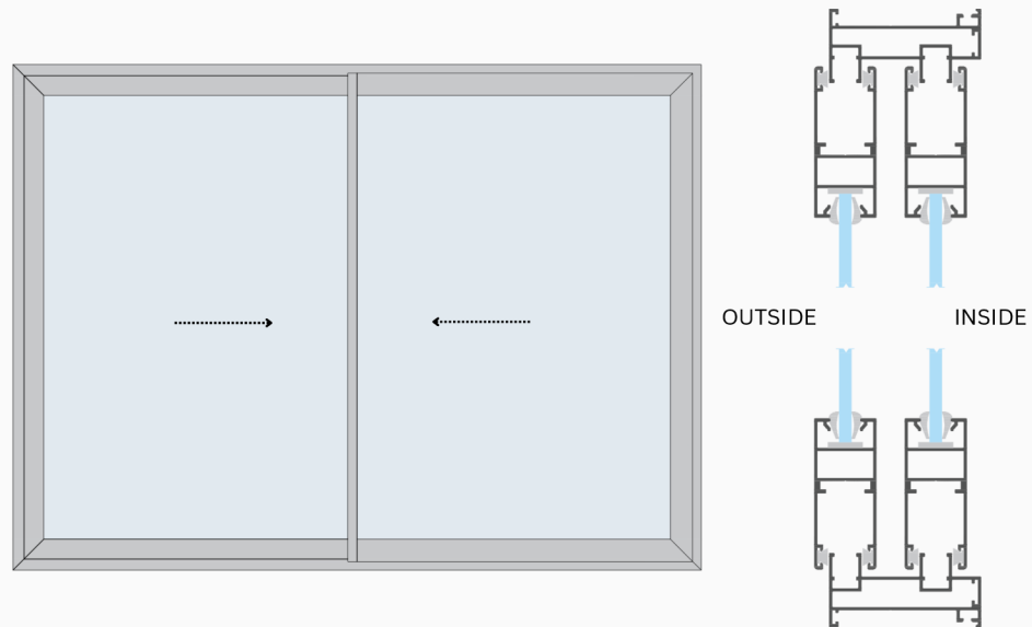
25mm FINE 2 TRACK SLIDING WINDOW
