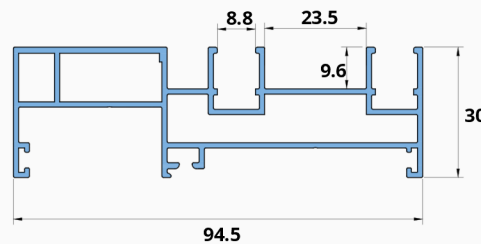
2 TRACK WITH GRILL Section Number - SA 103 Weight ( KG/M ) - 1.143
