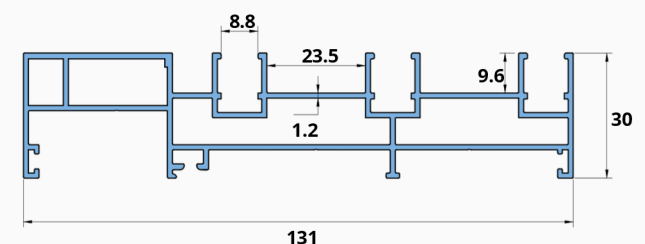
3 TRACK WITH GRILL Section Number - SA 104 Weight ( KG/M ) - 1.527
